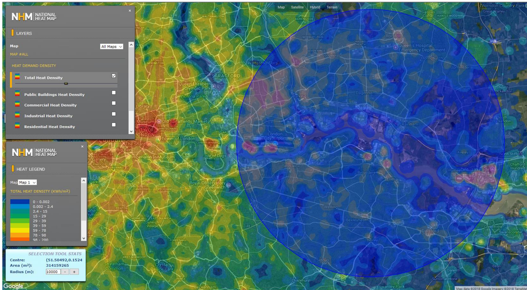
Figure 5: Local heat demand density, all sectors
